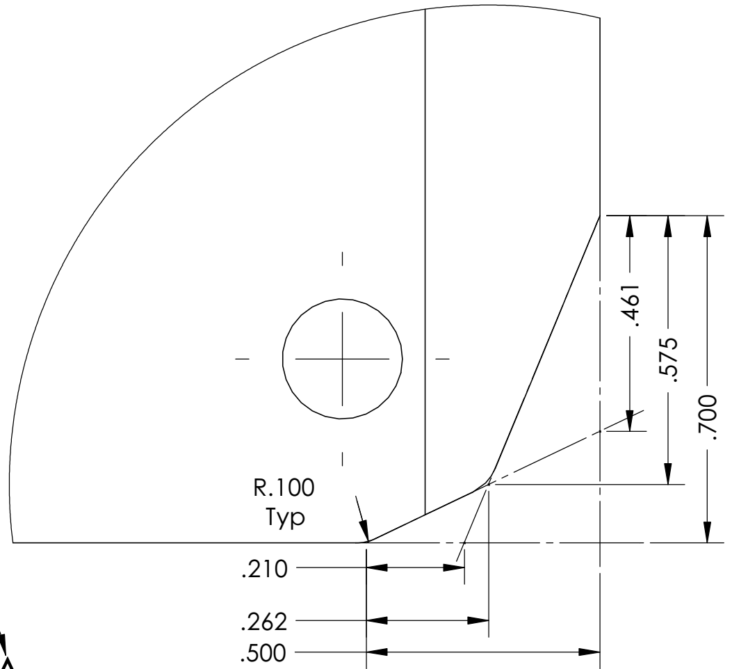
DETAIL A SCALE 3.5 : 1
