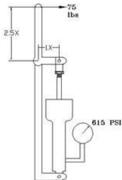
FIG 2 Minimum Geometry
