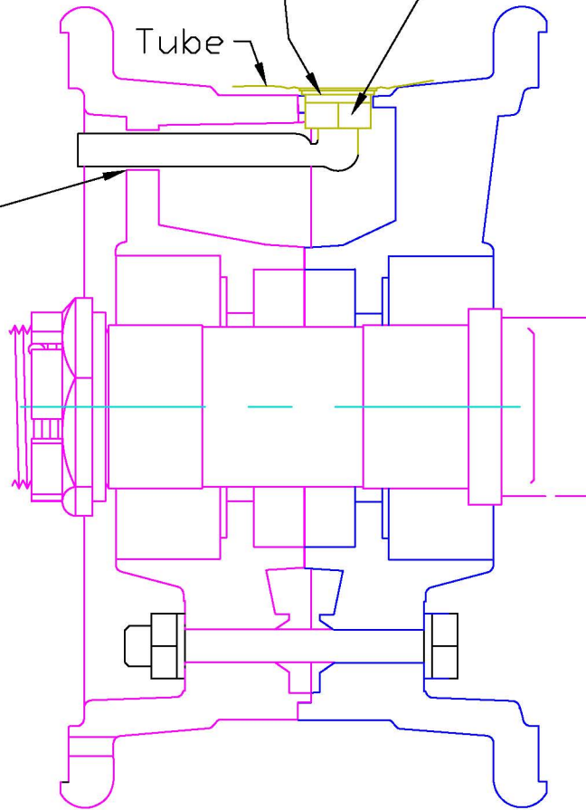
Tire Valve Installation
